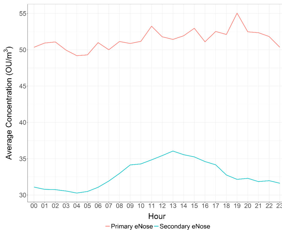
Figure 2-3 Diurnal trend of eNose odour measurements (2010-2017)
