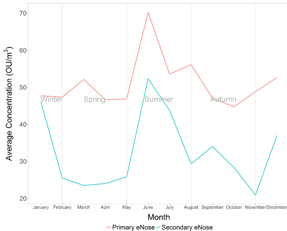
Figure 2-2 Seasonal trend of eNose odour measurements (2010-2017)
