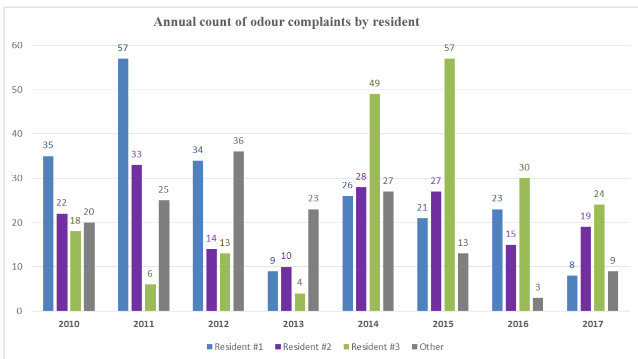
Figure 2-12 Annual count of odour complaints lodged against the RBCF by resident (2010-2017)
